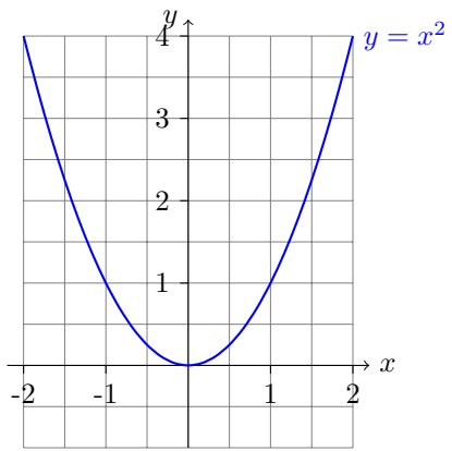
Figure 1: y = x^2
